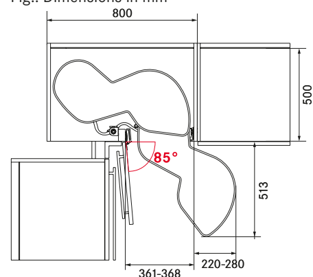
Fig.: Dimensions in mm
