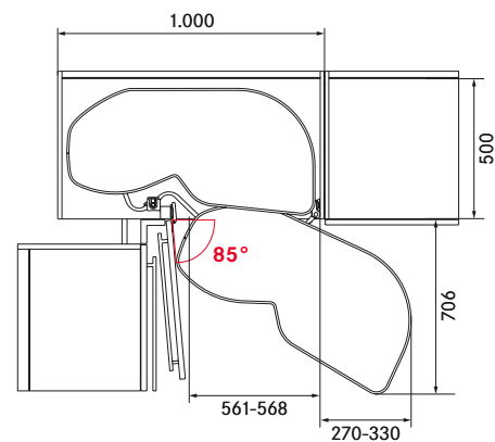
Example: swings out to the right (left cabinet – 60er Door)
