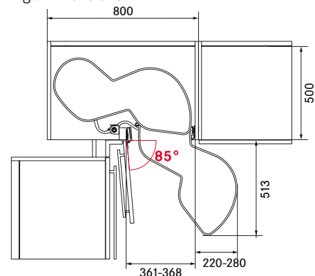
Example: swings out to the right (left cabinet – 40er Door)
