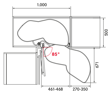
Example: swings out to the right (left cabinet – 50er Door)
