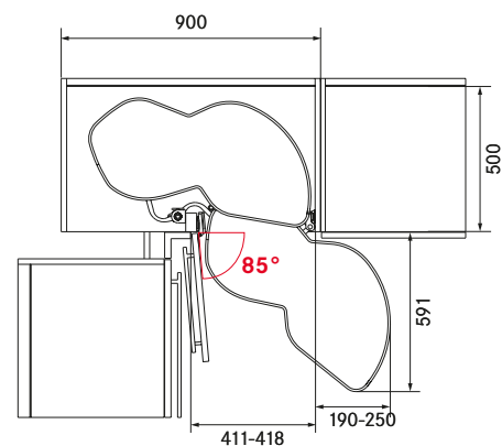
Example: swings out to the right (left cabinet – 45er Door)
